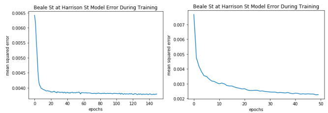
Fig. 3. Decreasing mean squared error (MSE) for Regression model training (left), and LSTM Network training (right) for the Beale St at Harrison St Ford GoBike station.
